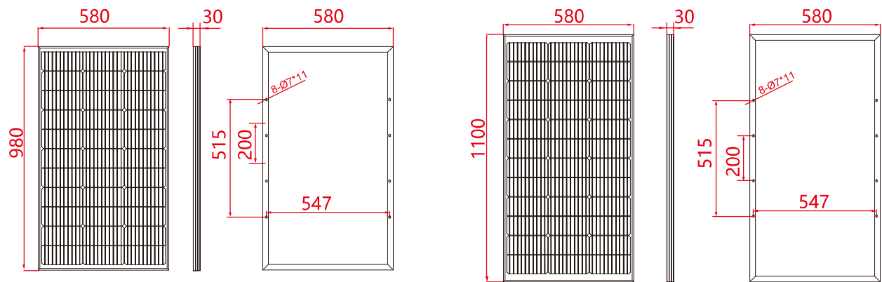
100W/18V
