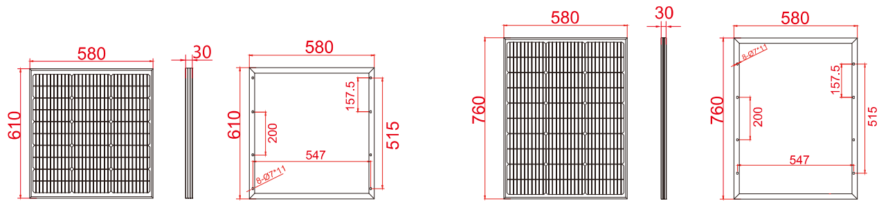
60W/6V
